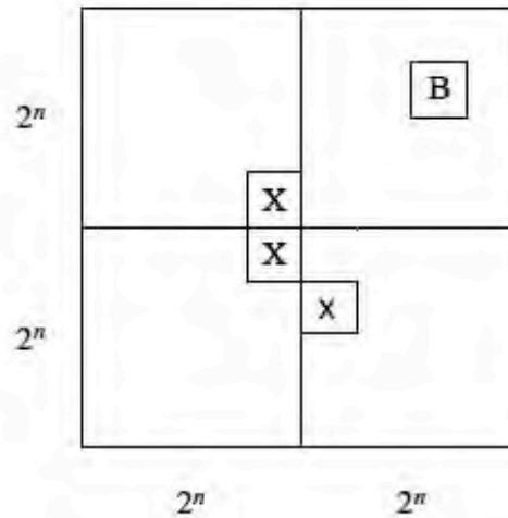
Figure 5.11 The induction hypothesis for the false theorem.
