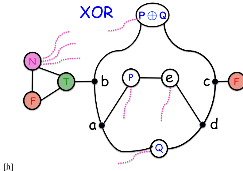
Figure 11.32 A 3-color XOR-gate
