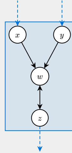
Figure 2: Addition gadget game. The dashed blue edges denote possible edges in the games, which are irrelevant to our result.
