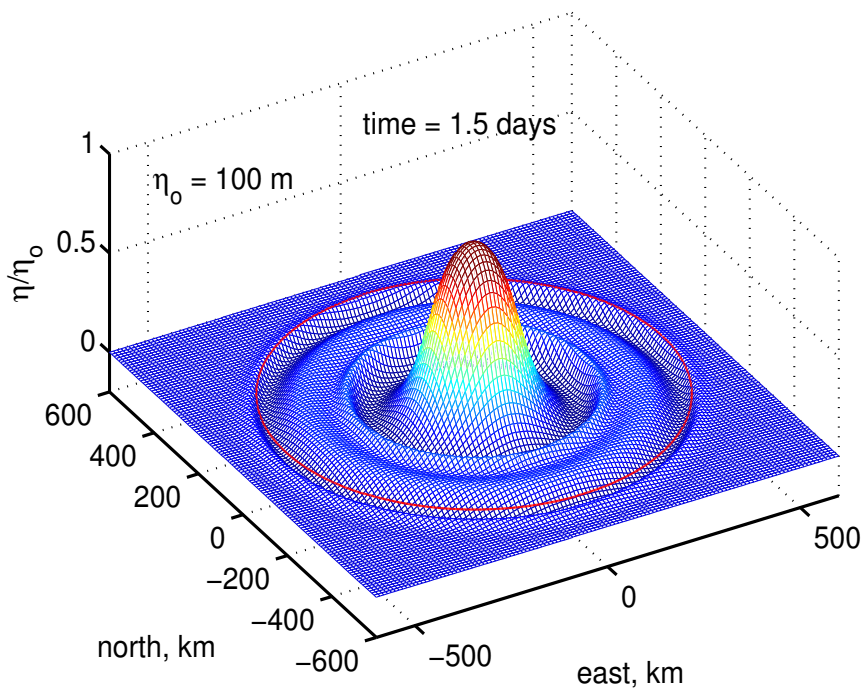
Figure 1: A snapshot taken 1.5 days after the start of a numerical experiment on geostrophic adjustment: a thickness anomaly of a dense fluid was released from rest onto an f -plane centered on 30^\circ\text{N} and allowed to evolve freely under the effects of gravity and rotation. The thickness anomaly slumps noticeably within the first half day, which excites inertia-gravity waves that expand isotropically. The leading edge propagates at the rate of a long, non-dispersive baroclinic gravity wave, roughly 275 \text{ km day}^{-1} in this case. After about ten days the inertia-gravity wave radiation was largely completed, leaving most of the height anomaly seen here in a near geostrophic balance. An animation of this experiment is online at https://scienceweb.who.edu/PO/people/jprice/education/ga2d-h100-f.mp4 The goal of this Part 2 essay is to understand how the geostrophic adjustment process varies with the environment, the radius of the initial height anomaly, and the initial potential vorticity.
